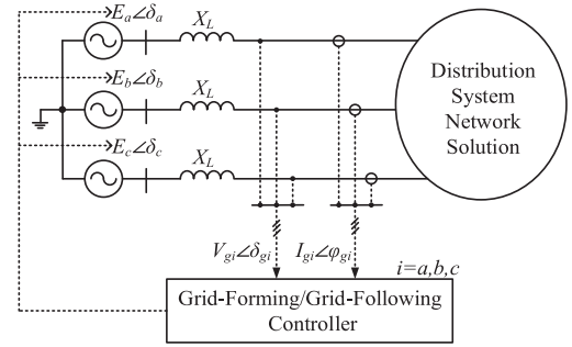
Fig. 5. Inverter equivalent circuit and controller.
