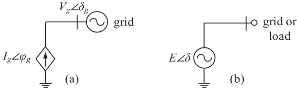
Fig. 4. Basic concepts of inverter controls: (a) grid-following and (b) grid-forming.
